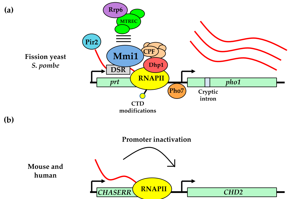
Figure 2. Gene expression control in cis by nearby lncRNAs. (a) In S. pombe , Mmi1 and additional protein factors, that are implicated in RNA processing and transcription regulation, associate with prt gene locus and lncRNA to affect expression of the downstream pho1 gene locus. (b) In mouse and human cells, the lncRNA CHASERR transcriptionally represses the downstream CHD2 gene through mechanisms that are currently unclear.
