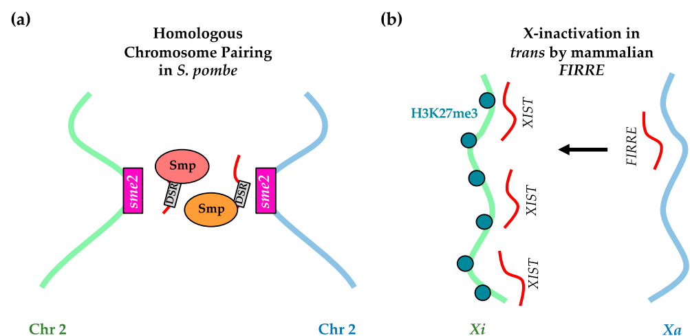
Figure 3. Intra-chromosomal regulation by long RNAs. (a) In S. pombe , DSR motif-containing RNAs from homologous chromosomes recruit sme2 -associating proteins (SMPs) to form nuclear clusters that help to bring the homologous chromosomes together. (b) In mammalian cells, the architectural
