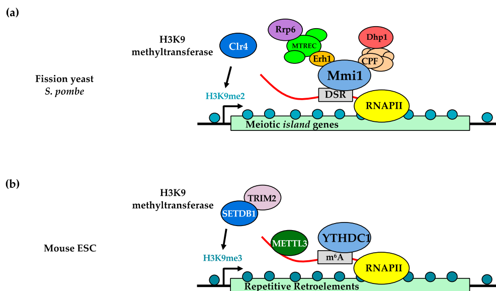
Figure 1. Histone H3 lysine 9 (H3K9) methylation promoted by YTH-family proteins. (a) In S. pombe , Mmi1 binds Determinant of Selective Removal (DSR) sequence motifs of meiotic RNAs derived from islands and engages with additional RNA processing and chromatin modification factors to trigger deposition of H3K9me2. (b) In mouse embryonic stem cells, YTHDC1 binds to certain m 6 A-modified RNAs to promote chromatin-association of m 6 A-writer METTL3. This promotes SETDB1/TRIM28-mediated deposition of repressive H3K9me3 modifications.
